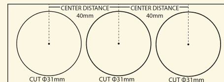
31mm CUTOUT EACH
